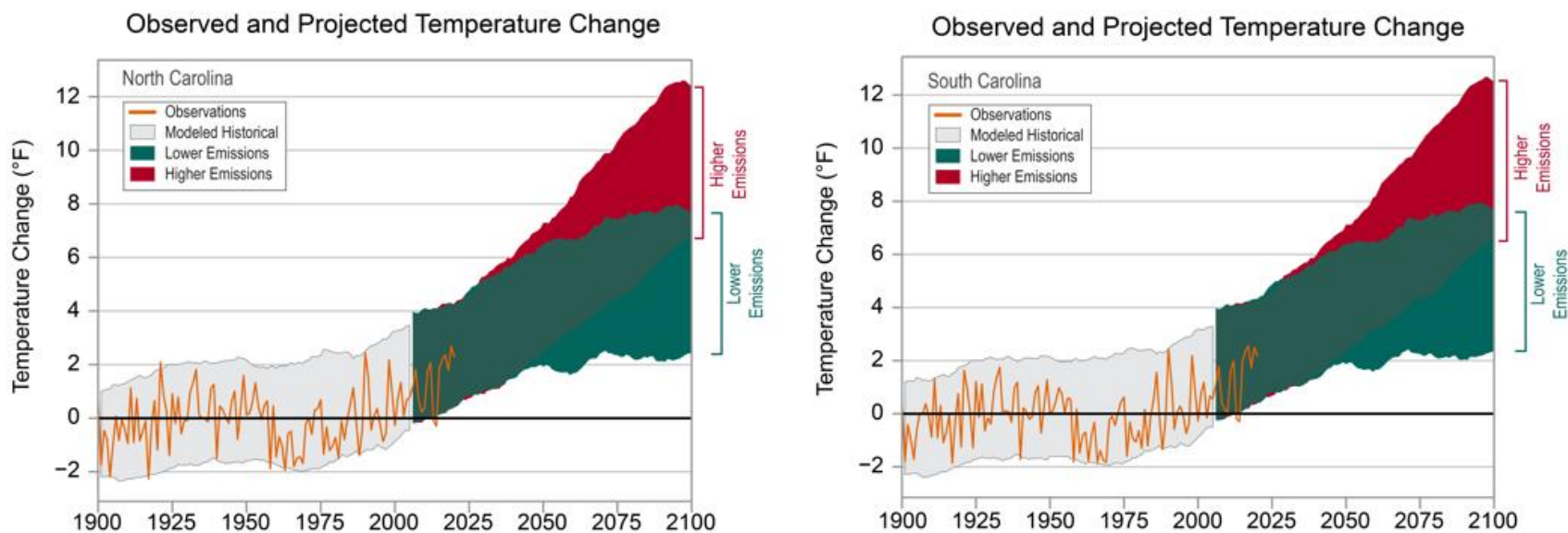
Figure 3-4. North Carolina and South Carolina average temperature historic trends and projections.
