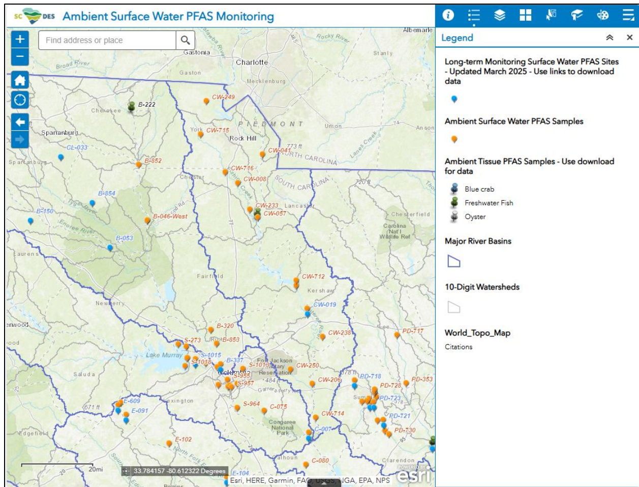
Figure 5-20. Ambient Surface Water PFAS project sampling sites
