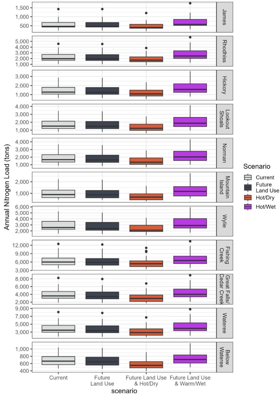
Figure 5-12. Annual Nitrogen Load by Reservoir Subbasin Under Current Conditions, Future Land Use, Future Land Use & Hot/Dry Climate, and Future Land Use & Warm/Wet Climate Scenarios Box shows 25 th percentile, median, and 75 th percentile
