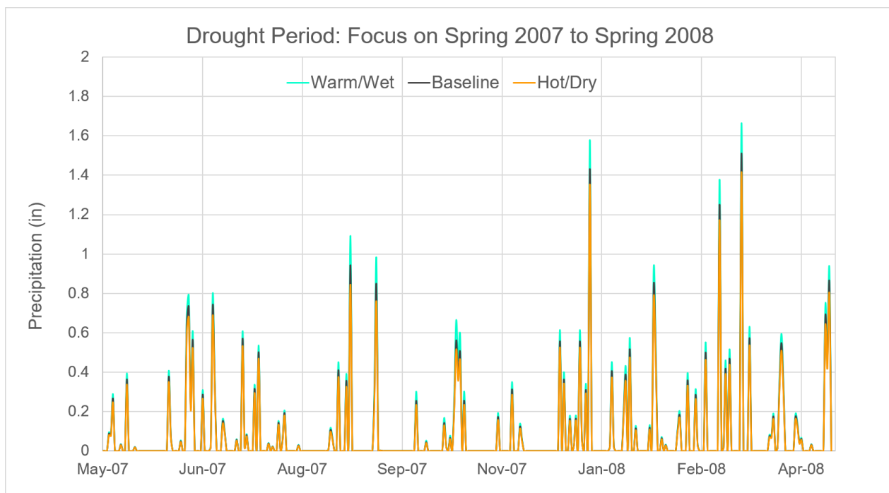
Figure 3-10. Daily Precipitation by Scenario During the May 2007 through April 2008 Period within the Multi-Year Drought
