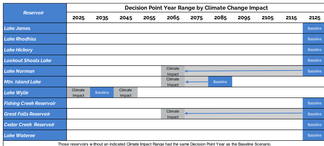
Figure 4-12. Decision Point Year Range for the Range of Climate Change Scenarios
